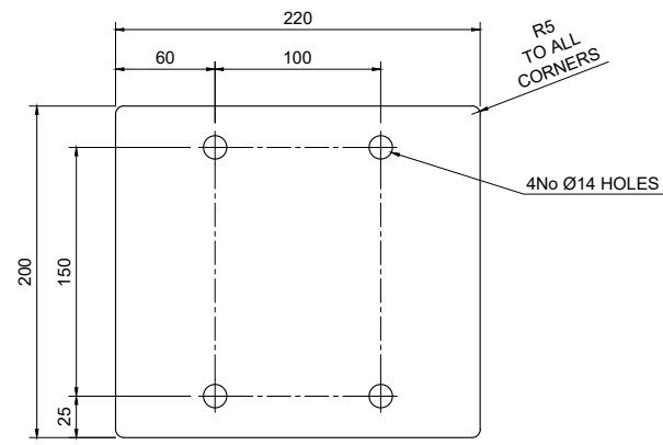
TPB-B-1 - 10mm THICK Scale 1:5
