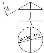
DETAIL A - TIMBER POLE TOP Scale 1:20
