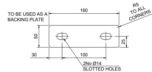
TPB-B-4 - 5mm THICK Scale 1:5
