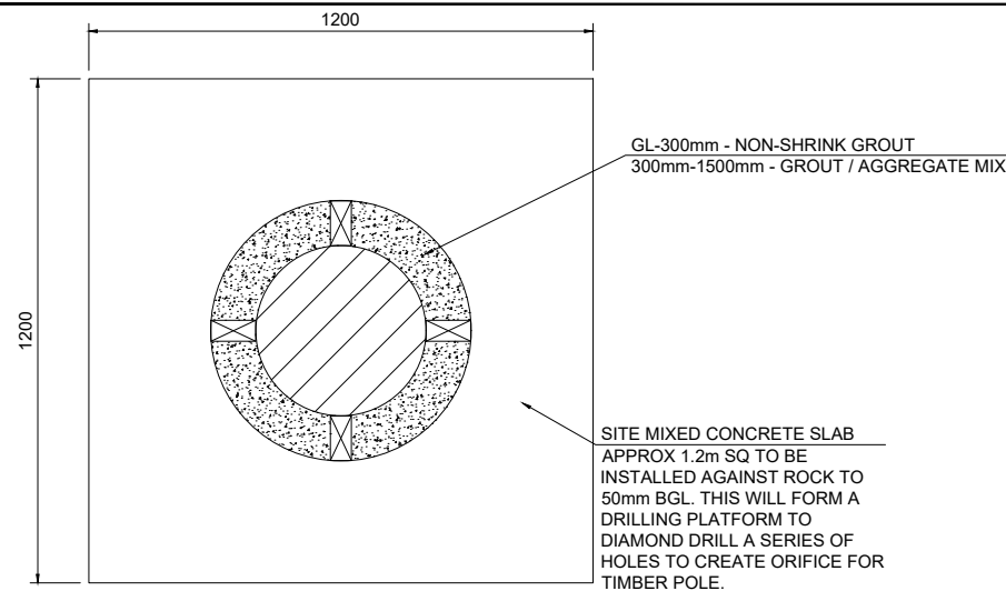
POROPOSED INSTALLATION PLAN VIEW Scale 1:20
