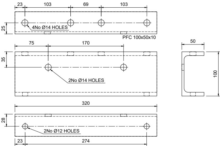
PART TPP-A-1 Scale 1:5
