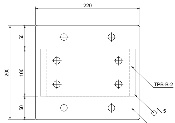
PART TPB-B Scale 1:5
