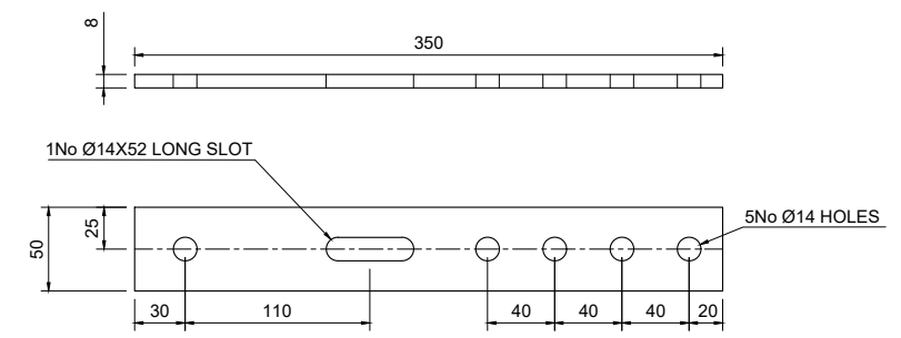
TPA-PD - 8mm THICK Scale 1:5
