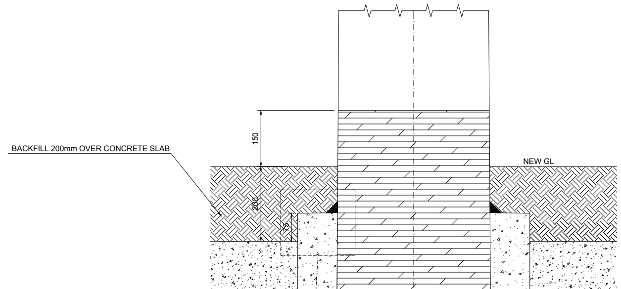
WATER PROOFING Scale 1:10
