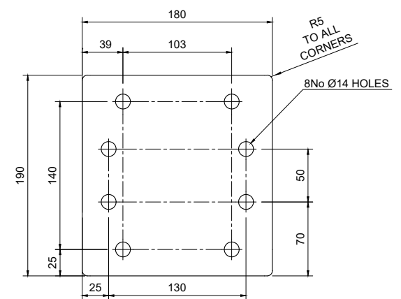
TPB-B-5 - 10mm THICK Scale 1:5
