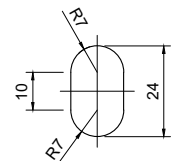
SLOTTED HOLE DETAIL Scale 1:2
