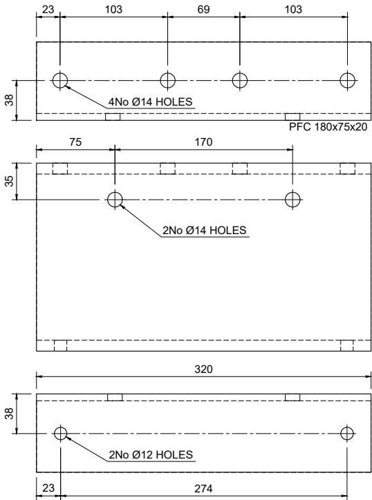
PART TPP-B-1 Scale 1:5
