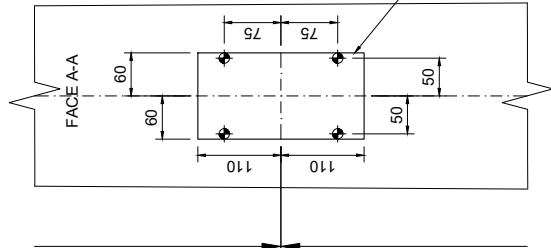
DETAIL 1 Scale 1:10
