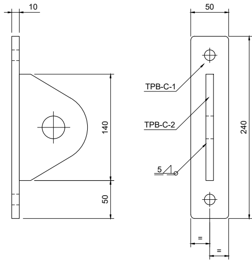
PART TPB-C Scale 1:5
