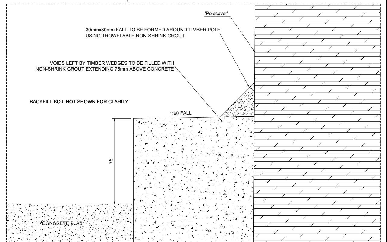
ENLARGED DETAIL Scale 1:2
