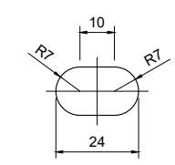
SLOTTED HOLE DETAIL Scale 1:2
