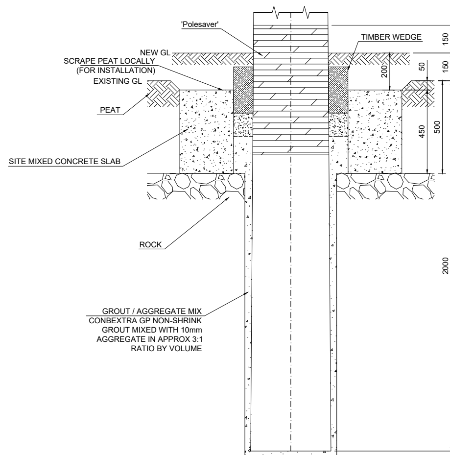
POROPOSED INSTALLATION ELEVATION Scale 1:20
