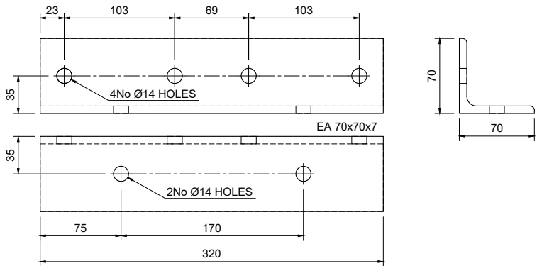
PART TPP-1 Scale 1:5
